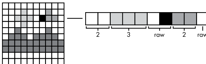
Figure 6-1: The selected row has a mix of runs and raw pixels.
